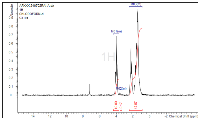
H-NMR Spectrum of copolymers in CDCl 3 (NMReady-60e, Nanalysis 60 MHz) NMR of PCL Copolymer
