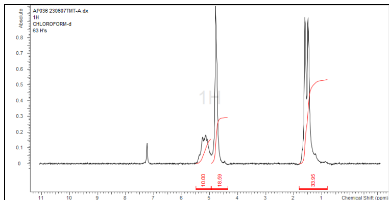
H-NMR Spectrum of copolymers in CDCl 3 (NMReady-60e, Nanalysis 60 MHz) NMR of PLGA Copolymer: LA:GA 55%:45% molar ratio (LA:GA 60%:40% w-w)
