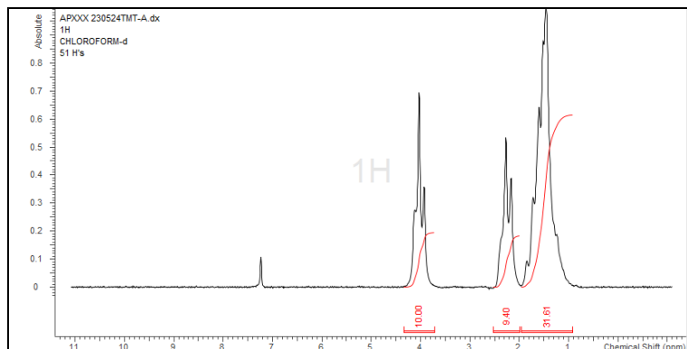
H-NMR Spectrum of copolymers in CDCl 3 (NMReady-60e, Nanalysis 60 MHz) NMR of PCL Copolymer
