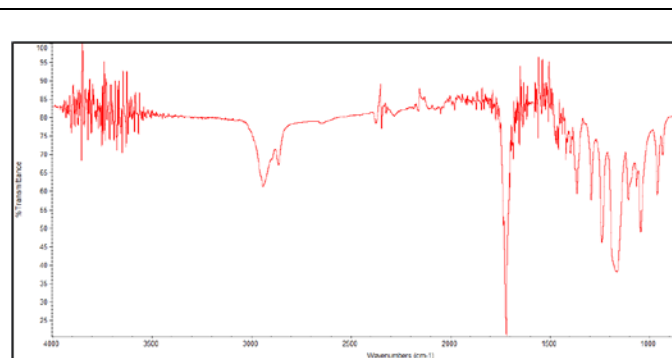
FTIR Analysis: Collected from IS5 ID7-ATR spectrometer (ThermoFisher) and analyzed in transmission mode.
