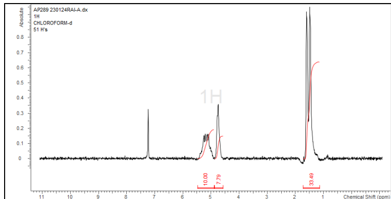
H-NMR Spectrum of copolymers in CDCl 3 (NMReady-60e, Nanalysis 60 MHz) NMR of PLGA Copolymer: LA:GA 72%:28% molar ratio (LA:GA 76%:24% w:w)
