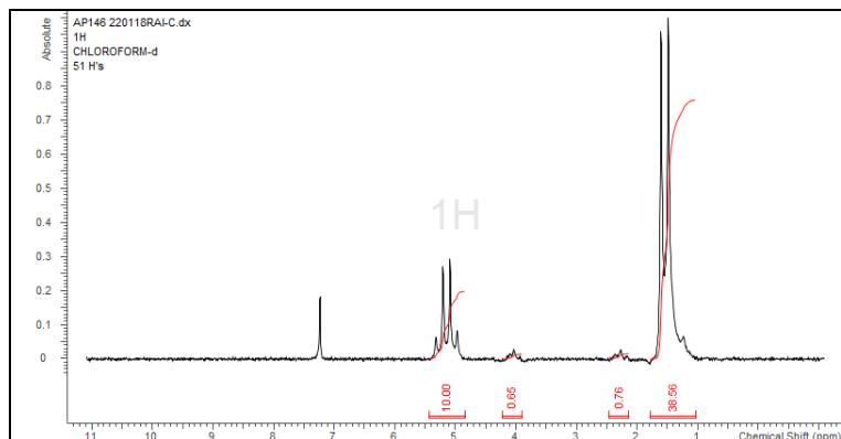
H-NMR Spectrum of copolymers in CDCl 3 (NMReady-60e, Nanalysis 60 MHz) NMR of P(L)LCL Copolymer: 97%-3% molar ratio (95%-5% w-w)
