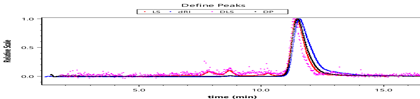
GPC-4D Analysis Method: Agilent 1260 Infinity II system 0.6 ml/min Acetone flow across TSKgel GMHHR-L, 7.8 mm x 30 cm. Detection Dawn Heleos II (MALLS), Optilab T-rex (RI), Dynapro nanostar (DLS), and Viscostar III (viscosity), universal calibration (Wyatt).
