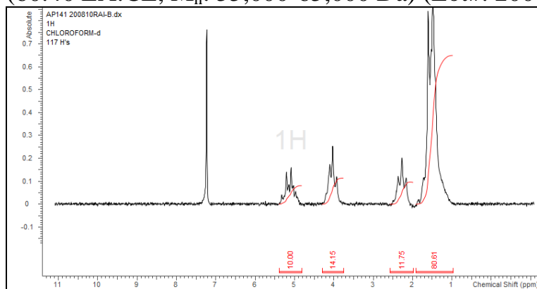
H-NMR Spectrum of copolymers in CDCl 3 (NMReady-60e, Nanalysis 60 MHz) NMR of PLGA copolymer: LA-GA = 59%-41% molar ratio (LA-GA 64%-36% w-w)
