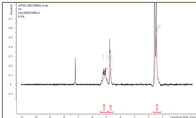
H-NMR Spectrum of copolymers in CDCl 3 (NMReady-60e, Nanalysis 60 MHz) NMR of PLGA copolymer: LA-GA = 69%-31% molar ratio (LA-GA 73%-27% w-w)
