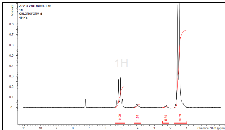
H-NMR Spectrum of copolymers in CDCl_3 (NMReady-60e, Nanalysis 60 MHz) NMR of PLCL Copolymer: LA-CL = 93%-7% molar ratio (LA-CL 89%-11% w-w)
