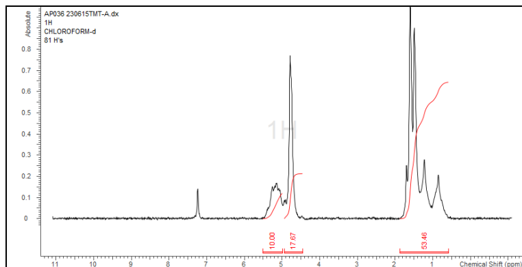
H-NMR Spectrum of copolymers in CDCl 3 (NMReady-60e, Nanalysis 60 MHz) NMR of PLGA Copolymer: LA:GA 53%-47% molar ratio (LA:GA 42%:58% w-w)
