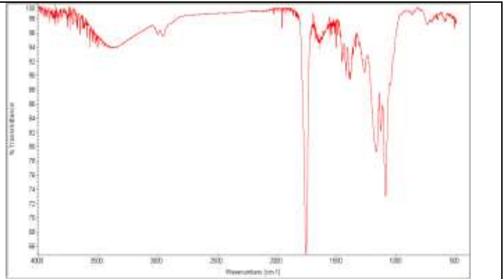
FTIR Analysis: Collected from cast-film on salt-plate placed in Protégé 460 Spectrometer (Nicolet) and analyzed in transmission E.S.P. mode.
