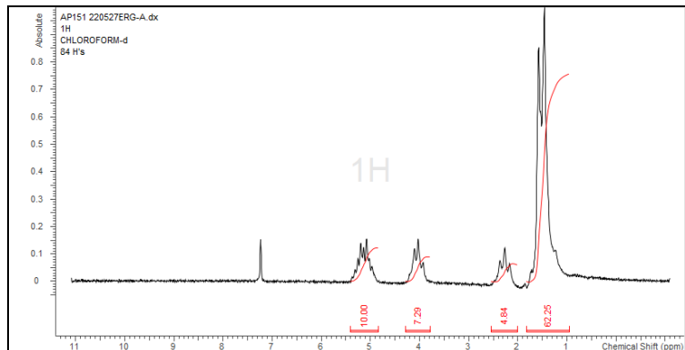
H-NMR Spectrum of copolymers in CDCl 3 (NMRReady-60e, Nanalysis 60 MHz) NMR of PLCL Copolymer: LA:CL 73%:27% molar ratio (LA:CL 63%:37% w-w)
