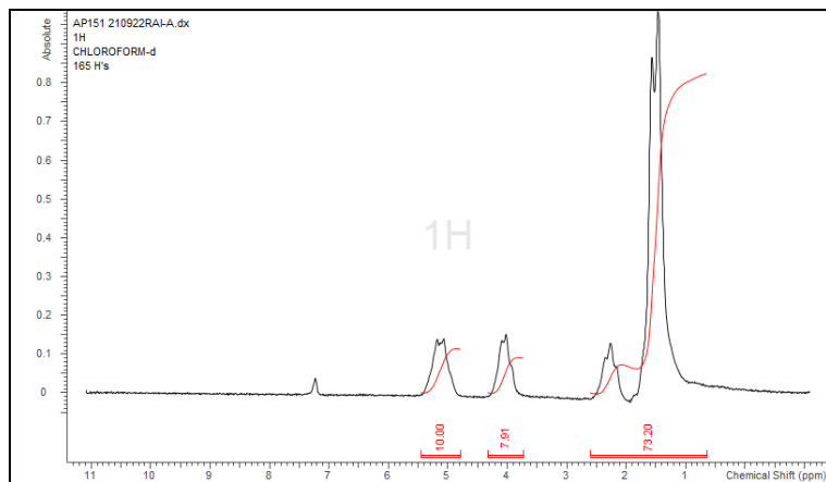
H-NMR Spectrum of copolymers in CDCl 3 (NMReady-60e, Nanalysis 60 MHz) NMR of PLCL Copolymer: 72%-28% molar ratio (61%-39% w-w)
