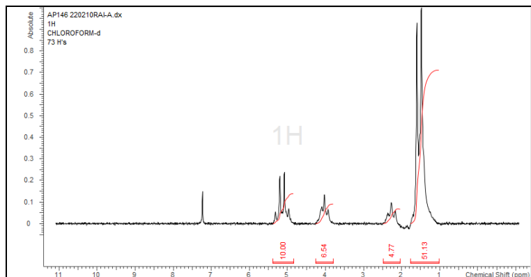
H-NMR Spectrum of copolymers in CDCl 3 (NMReady-60e, Nanalysis 60 MHz) NMR of P(L)LCL Copolymer: 75%-25% molar ratio (88%-12% w-w)
