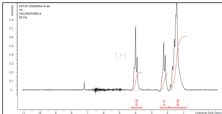
H-NMR Spectrum of copolymers in CDCl 3 (NMRReady-60e, Nanalysis 60 MHz) NMR of PCL Copolymer
