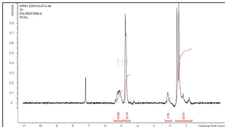
H-NMR Spectrum of copolymers in CDCl 3 (NMReady-60e, Nanalysis 60 MHz) NMR of PLGA Copolymer: LA-GA 47%-53% molar ratio (LA-GA 53%-47% w-w)
