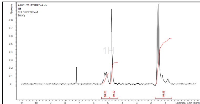
H-NMR Spectrum of copolymers in CDCl 3 (NMReady-60e, Nanalysis 60 MHz) NMR of PLGA Copolymer: LA-GA 51%-49% molar ratio (LA-GA 56%44% w-w)
