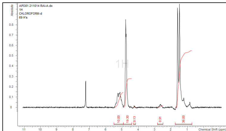
H-NMR Spectrum of copolymers in CDCl 3 (NMReady-60e, Nanalysis 60 MHz) NMR of PLGA Copolymer: 51%-49% molar ratio (56%-44% w-w)
