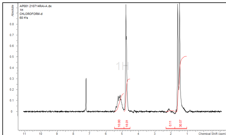
H-NMR Spectrum of copolymers in CDCl 3 (NMReady-60e, Nanalysis 60 MHz) NMR of PLGA Copolymer: LA:GA 53%:47% molar ratio (58%:42% w:w)
