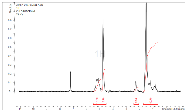
H-NMR Spectrum of copolymers in CDCl 3 (NMReady-60e, Nanalysis 60 MHz) NMR of PLGA Copolymer: 52%:48% molar ratio (57:43% w:w)
