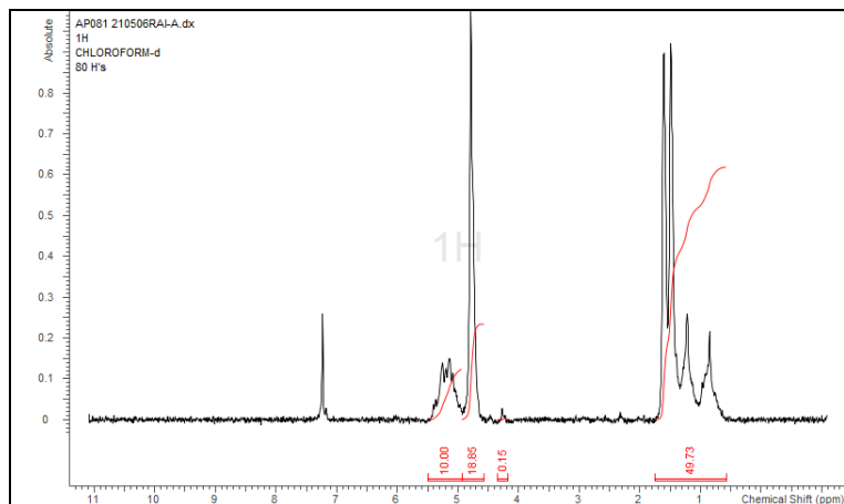
H-NMR Spectrum of copolymers in CDCl 3 (NMReady-60e, Nanalysis 60 MHz) NMR of PLGA Copolymer: LA-GA = 51%-49% molar ratio (LA-GA 57%-43% w-w)
