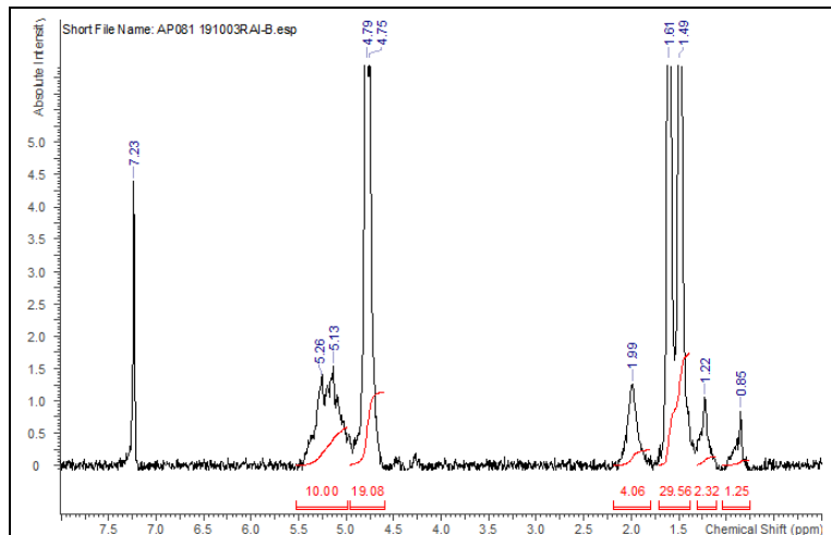
H-NMR Spectrum of copolymers in CDCl 3 (NMReady-60e, Nanalysis 60 MHz) NMR of PLGA copolymer: LA-GA = 51%-49% molar ratio (LA-GA 57%-43% w-w)
