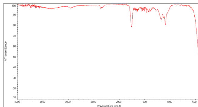
FTIR Analysis: Collected from cast-film on KBr salt-plate placed in a Nicollet Avatar 320 spectrometer and analyzed in transmission mode.
