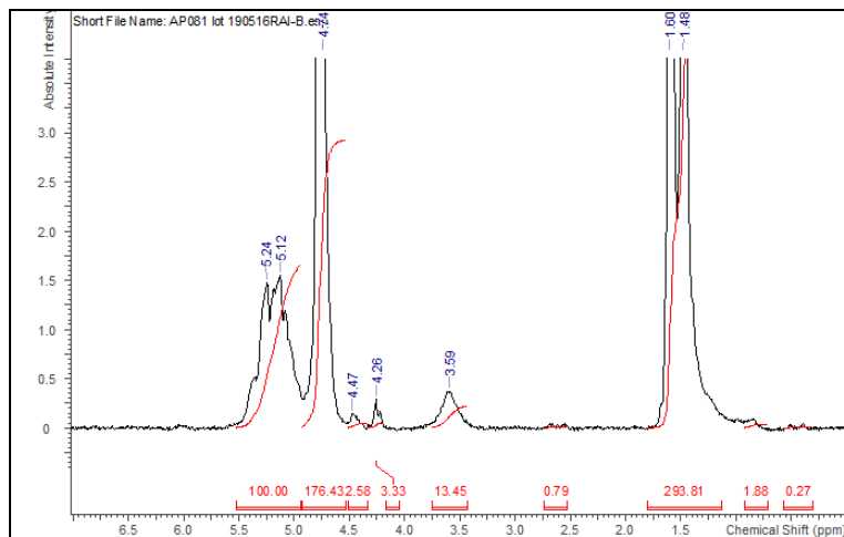
H-NMR Spectrum of copolymers in CDCl 3 (NMReady-60e, Nanalysis 60 MHz) NMR of PLGA copolymer: LA-GA =53%/47% molar ratio (LA:GA 58%/42% w/w)
