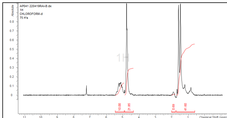
H-NMR Spectrum of copolymers in CDCl 3 (NMReady-60e, Nanalysis 60 MHz) NMR of PLGA Copolymer: LA-GA 48%-52% molar ratio (LA-GA 53%-47%)
