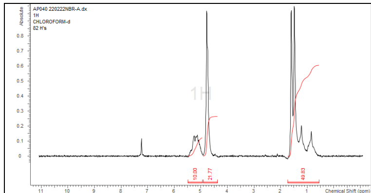
H-NMR Spectrum of copolymers in CDCl 3 (NMReady-60e, Nanalysis 60 MHz) NMR of PLGA Copolymer: 48%-52% molar ratio (53%-47% w-w)
