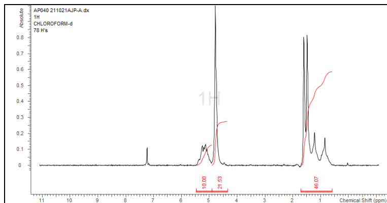
H-NMR Spectrum of copolymers in CDCl 3 (NMReady-60e, Nanalysis 60 MHz) NMR of PLGA Copolymer: LA-GA 48%-52% molar ratio (54%-46% w-w)
