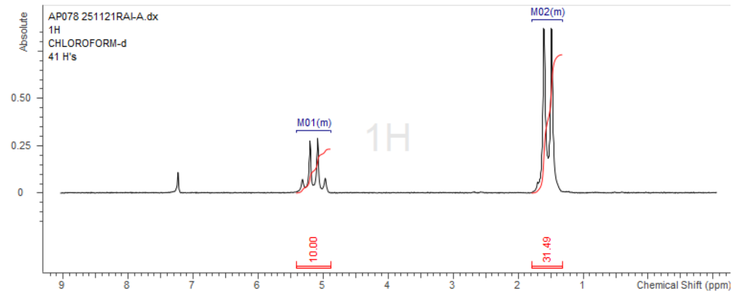
H-NMR Spectrum of copolymers in CDCl_3 (NMReady-60e, Nanalysis 60 MHz) NMR of PLLA
