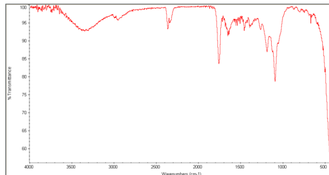
FTIR Analysis: Collected from cast-film on KBr salt-plate placed in a Nicollet Avatar 320 spectrometer and analyzed in transmission mode.
