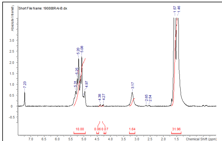
H-NMR Spectrum of copolymers in CDCl 3 (NMReady-60e, Nanalysis 60 MHz) NMR of PDLLA copolymer.
