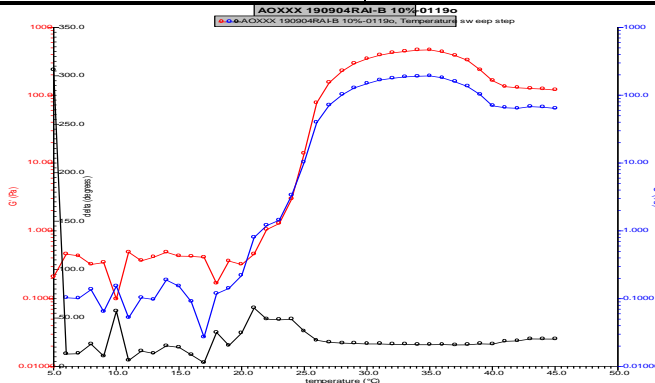
Rheology performed on AR2000 (TA instruments) with 60mm 2degree cone on 10% w/v polymer in water dissolved over 3 days with stirring at 4°C. Viscosity of solution at 0.1 (sec -1 ) and 5°C was measured (1minute peak hold 5 second test intervals). Rheology performed by oscillating at constant 6.283 rad/s, 0.1% strain, in increments of 1°C ranging from 5-45°C with 1 minutes of temperature equilibration at each point.
