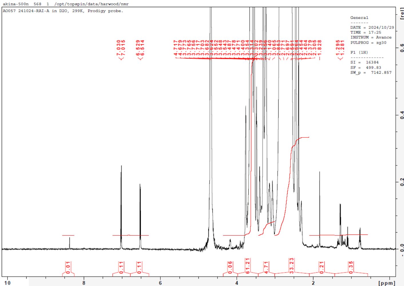
H-NMR Spectrum of copolymers in D 2 O (NMReady-60e, Nanalysis 60 MHz) NMR of PEG-PEI copolymer
