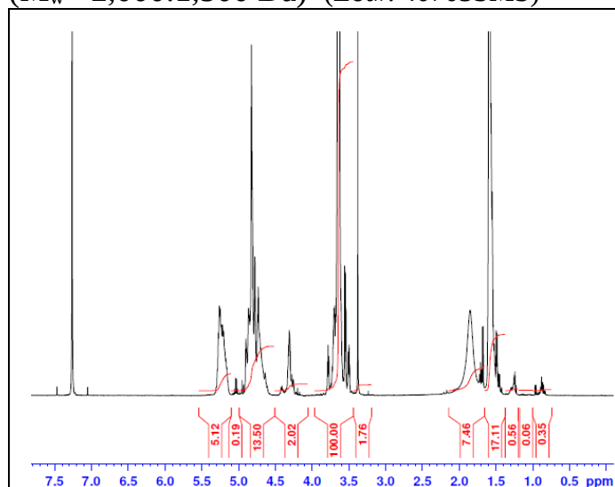
1 H-NMR Spectrum of mPEG-PLGA copolymer in CDCl 3 (Varian Inova 500 MHz instrument), NMR of mPEG-PLGA repeat units: EG-LA/GA = 45-9/12 ( M_n EG-LA/GA = 1982-664/705)
