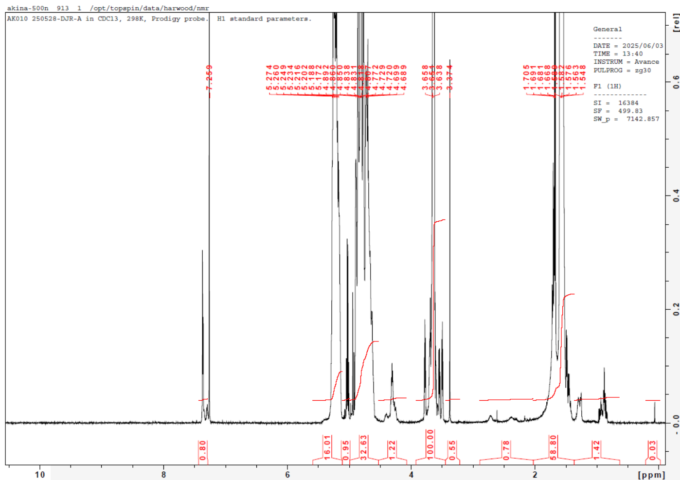
H-NMR Spectrum of copolymers in CDCl 3 (Bruker ≥300 MHz, PINMRF) NMR of PLGA-PEG copolymer: EG/LA-GA =109*/70-71 molar ratio (Mn EG/LA:GA 4802*/5026-4129 Da) LA:GA 55%:45%
