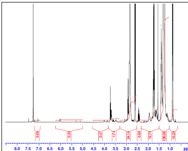
H-NMR Spectrum of copolymers in CDCl 3 (Varian Inova 500 MHz instrument) NMR of C18-NHS
