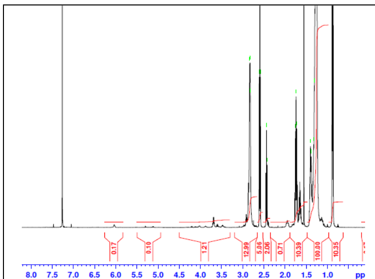
H-NMR Spectrum of copolymers in CDCl 3 (Varian Inova 500 MHz instrument) NMR of C18-NHS
