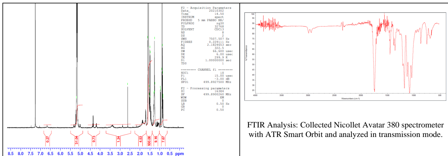
H-NMR Spectrum of copolymers in CDCl 3 (Bruker ≥300 MHz, PINMRF) NMR of PLLA-NH 2 copolymer.
