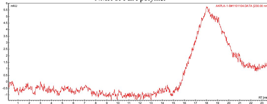
GPC analysis of PLA polymer
