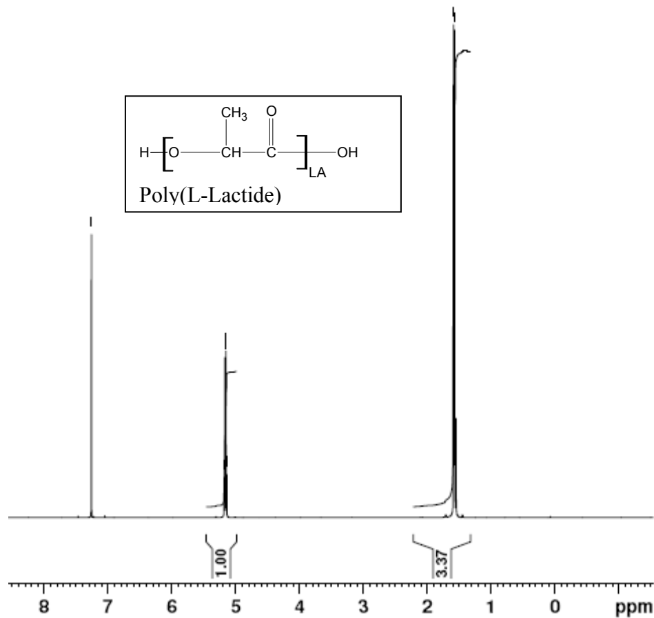
NMR of PLLA polymer – 100% Lactide:0%Glycolide
