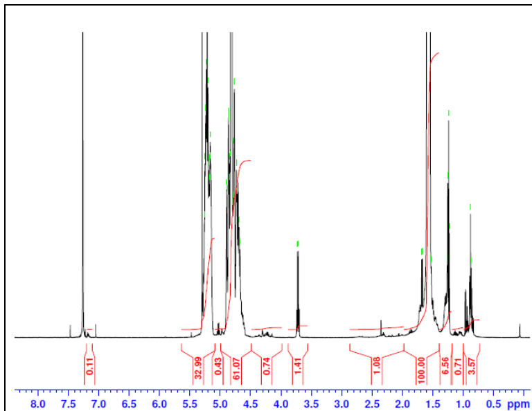
H-NMR Spectrum of PLGA copolymers in CDCl 3 (Varian Inova 500 MHz instrument), NMR of PLGA copolymers: LA/GA = 57%/43%
