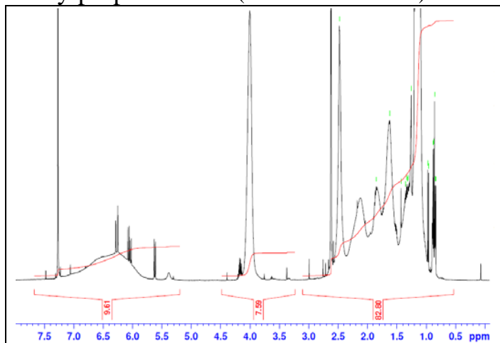
H-NMR Spectrum of PNIPAM copolymers in CDCl 3 (Varian Inova 500 MHz instrument),
