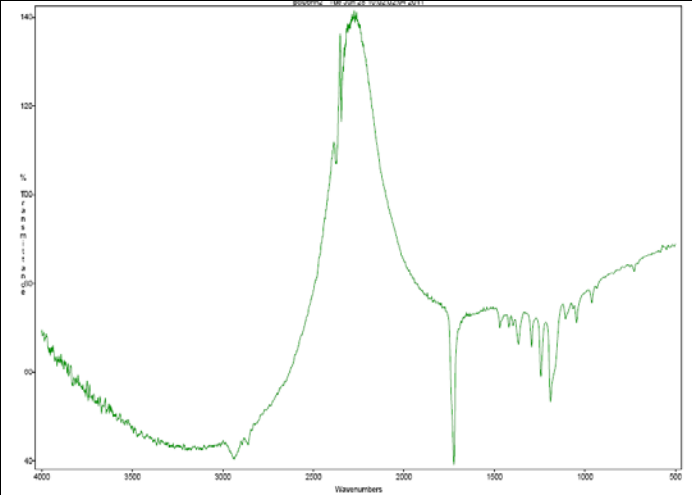
FTIR Analysis: Collected from cast-film on KBR salt-plate placed in Sattelite FTIR (Thermo-Mattson) and analyzed in transmission mode.
