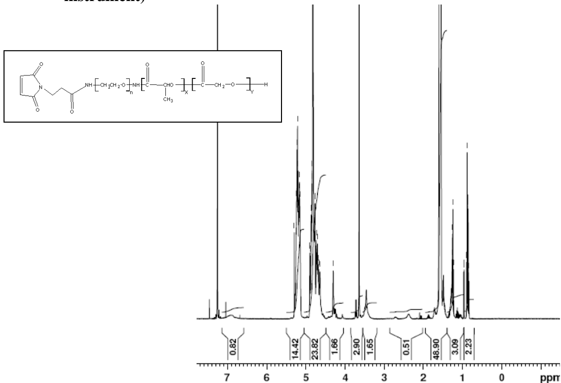
M n , NMR of Mal-PEG-PLA/PGA copolymers
